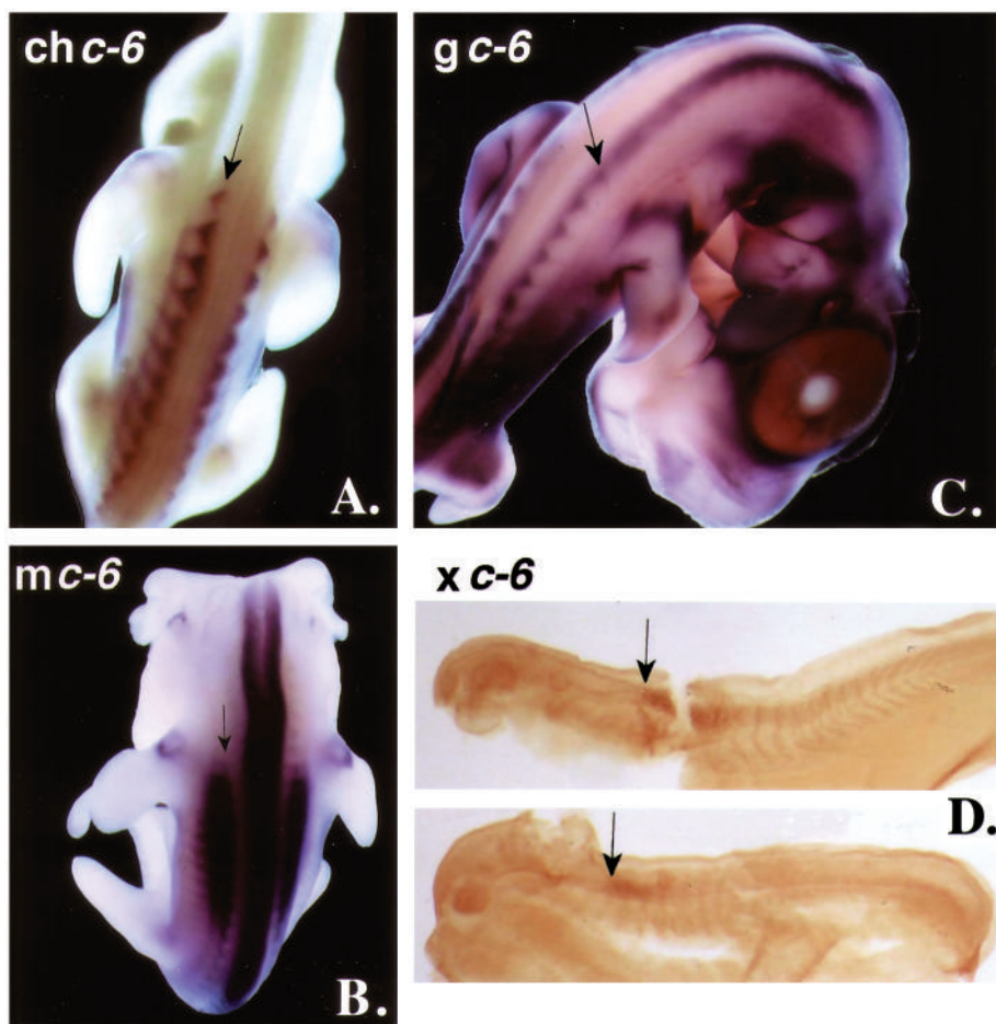
Fig. 5. Whole-mount in situ hybridizations with members of paralogue 6. Arrows indicate the anterior limit of gene expression in the paraxial mesoderm. (A) Chick (st. 25) Hoxc-6 expression boundary lies at somite level 19-20, aligned with the middle of the forelimb, at the first thoracic vertebra (T1). The paraxial mesoderm is labeled in an 'arcade' pattern along the flank: intersegmental labeling forms arches that meet dorsally in mid-segment, defining each somite. Somite labeling continues posteriorly into the tail. Laterally in the mid-flank there is a band of nearly continuous expression running anterior-posterior along the original boundary between somitic and lateral plate mesoderm. Lateral to this, in the body wall are streaks of inter segmental expression that trace the myosepta. (B) Mouse (E12) Hoxc-6 expression is aligned with the middle of the forelimb at somite level 12-13, the first thoracic vertebra, consistent with data reported by Jegalian et al. (1992). The mouse does not show an 'arcade' pattern of expression but the label is very strong in a near-continuous region of trunk mesoderm that covers approximately eight segments and extends laterally to the horizontal septum. Ventrally, the label is inter segmental, tracing the myosepta and rib positions in the body wall. (C) Goose at the morphological equivalent of a stage 25-26 chick embryo hybridized with chick the Hoxc-6 probe. Two different probes were used, both giving positive results with a variable degree of background that is comparable in chick and goose embryos. The labeling pattern is very similar to that of the chick including anterior-proximal limb labeling reported elsewhere (Sharp et al. 1988; Nelson et al. unpublished data), and a partial arcade pattern of somitic labeling. The paraxial mesoderm labeling starts at an axial level that aligns with the middle of the forelimb, at somite level 22-23, the first thoracic vertebra. (D) Whole-mount immunohistochemistry with XlhbBox-1 antibody on stage 35 Xenopus embryos. Labeling begins at the border between somite 3 and somite 4, forming a continuous border across the neural tube and the mesoderm in agreement with labeling reported by Oliver et al. (1988).
